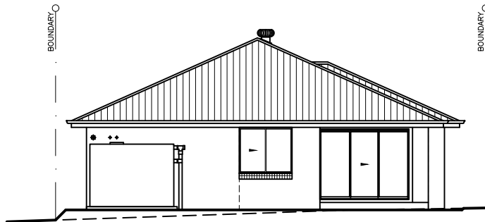
ELEVATION D (SOUTH)
